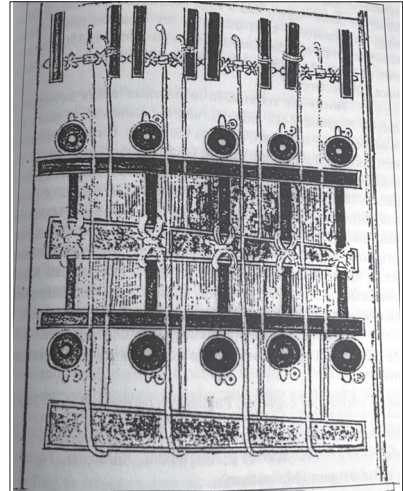
FIG. 3.4 Ashokan pillar hauled by means of rope and capstan from ground on to a ten-wheel cart. Diagram in Sirat-i Firozshahi MS. (Courtesy: Khuda Bakhsh Oriental Public Library, Patna.) There are ten other diagrams in the same manuscript, illustrating its account of transport of the pillar from Topra to Delhi, fourteenth century.
