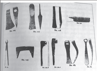
Fig. 13 Iron tools from Taxila: axe (no. 103); adze (no. 112); chisel (no. 118); knife (no. 122); tongs (no. 130); anvil (no. 143); nails (nos. 150a and b); hoes (nos. 183 and 184); Bhir Mound, Stratum II (except no. 112, which is from the lower Stratum III). (Reprod. J. Marshall)
